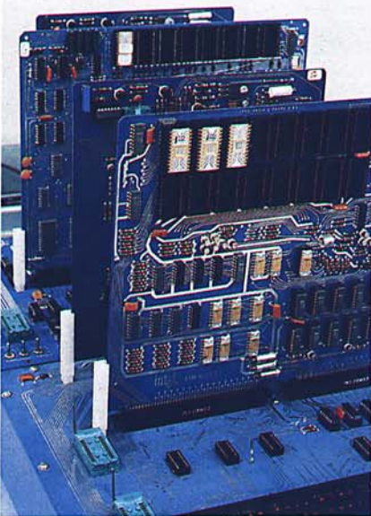
Shortly after the introduction of the 4004 microprocessor, Intel began offering design aids to help customers develop 4004-based products. The rather primitive-looking devices shown here are the MCB 410 connector board with the SIM 4-01 prototyping board and the MB7-02 PROM programming board, manufactured in 1972.
