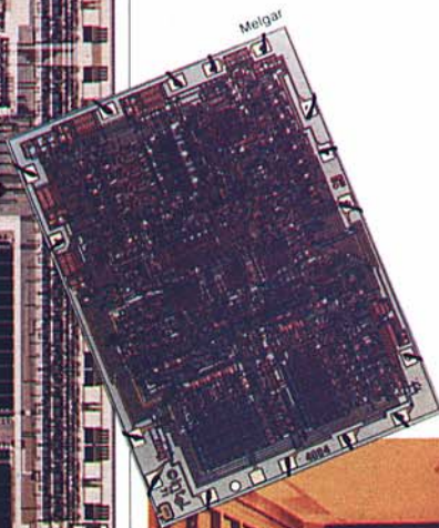
Relative sizes of the 80286 (left) and 4004 microprocessors are shown. The 4004, introduced in 1971, measures 117 X 159 mils (thousandths of an inch) and incorporates about 2300 transistors. The 80286, introduced in 1982, measures 342 X 347 mils and incorporates 130,000 transistors. Microprocessors have far more computing power than ENIAC (below), the first electronic computer, which was built in 1946.
