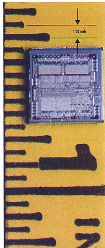
Actual size of Intel's 80C51 microcontroller, which is manufactured using Intel's high-performance, low-power CHMOS process.
