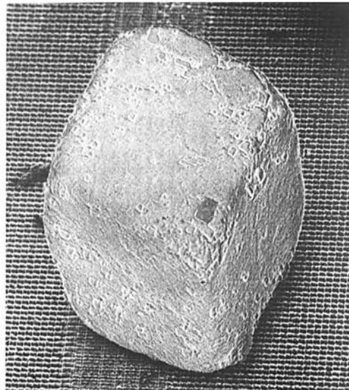
Scanning Electron Microscopic view of a common table salt crystal resting on Intel's high-density 27128 EPROM. Each of the 27128's 131,072 cells measures approximately 7 microns (7 millionths of a meter) across, in contrast to the average salt crystal's 300 microns.
